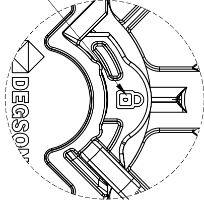
View A 4:1
